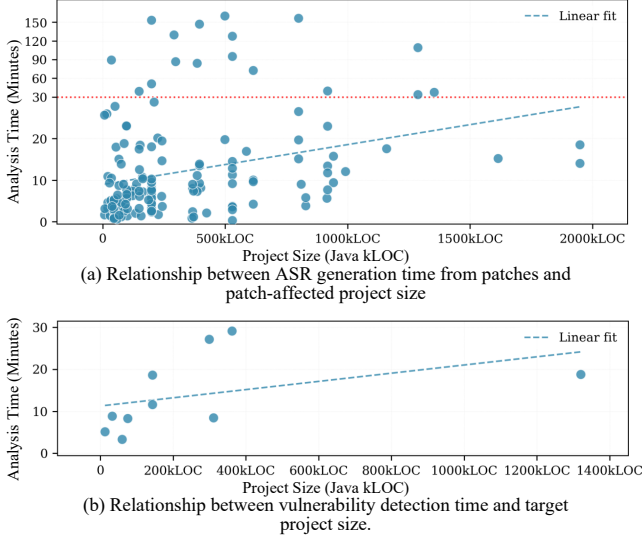
Figure 10: Relationship between VULGENIE’s analysis time and project size.
