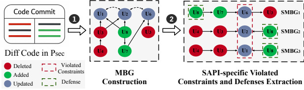
Figure 5: MBG construction and violated constraints and defenses extraction.
