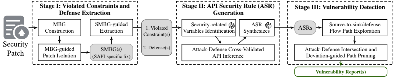
Figure 4: The Overall Architecture of VULGENIE with Three Stages.
