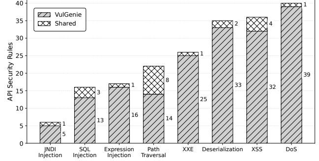
Figure 9: Distribution and Overlap of SAPIs Extracted by VULGENIE vs. CodeQL Across eight Vulnerability Types (Shared means SAPIs that are commonly owned)
