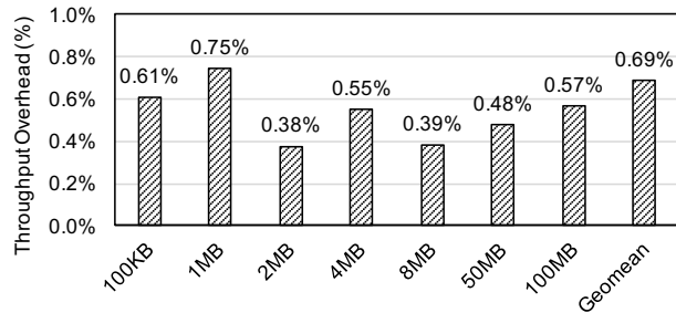
Figure 7: Throughput overhead of Cherokee server.
